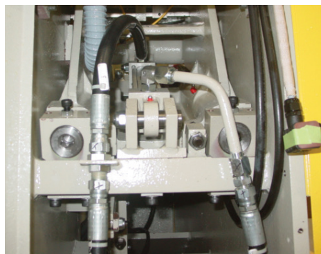
AFTER REMANUFACTURE
